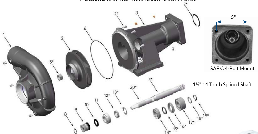
101-B69875 Pump shown here on an 8,000 Gallon, Volvo A40G Tank System Manufactured by Tidal Wave Tanks, Mulberry Florida
